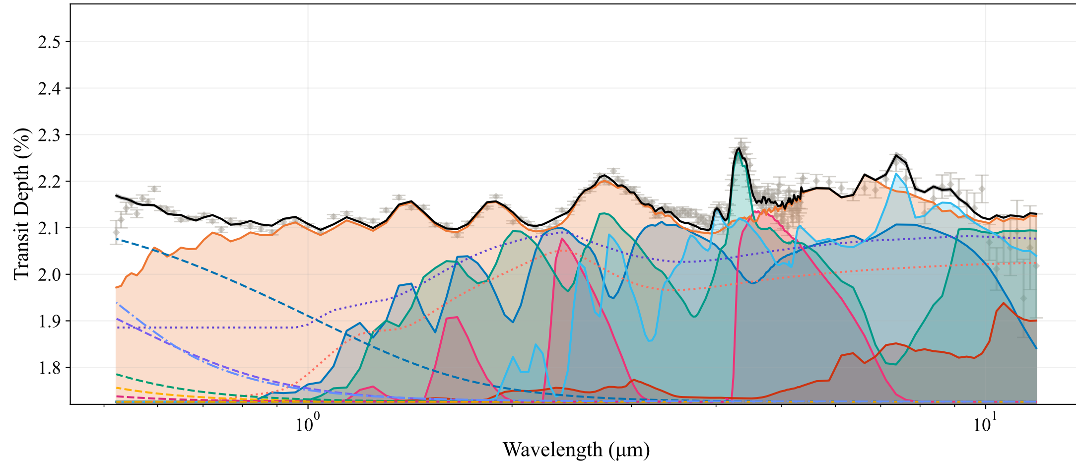
PRISM + MIRI, SO2 + Na2S
